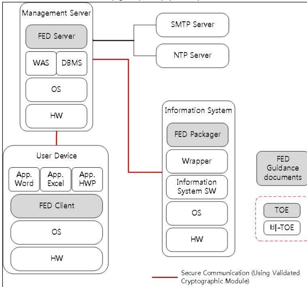
[Figure 2] TOE's physical scope
