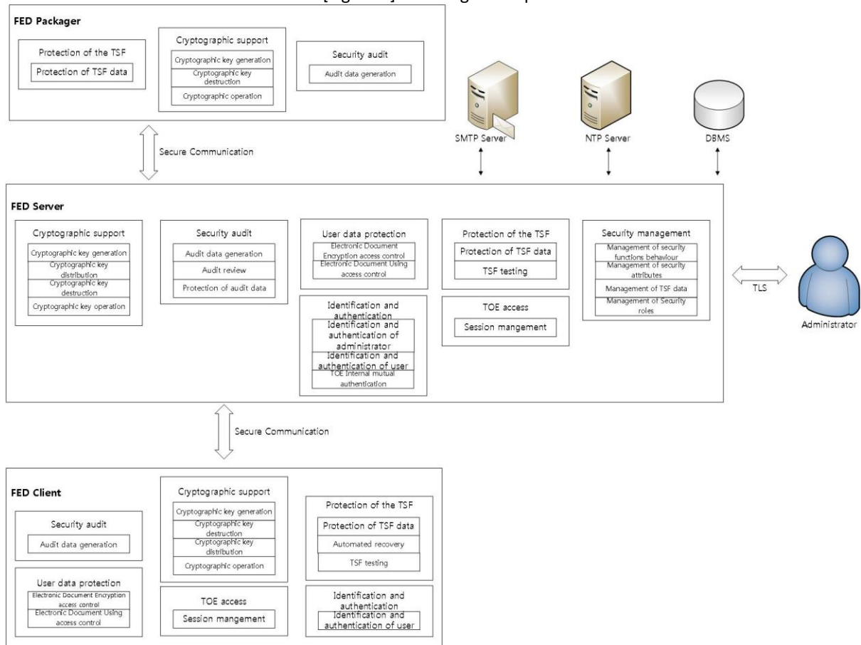
[Figure 3] TOE's logical scope
