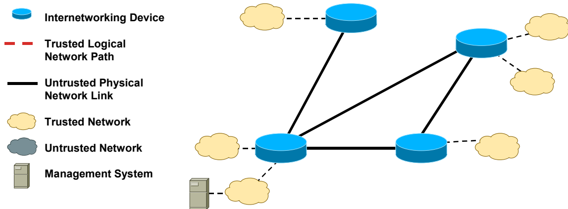
Figure 2-14 - Insecure Intranet
