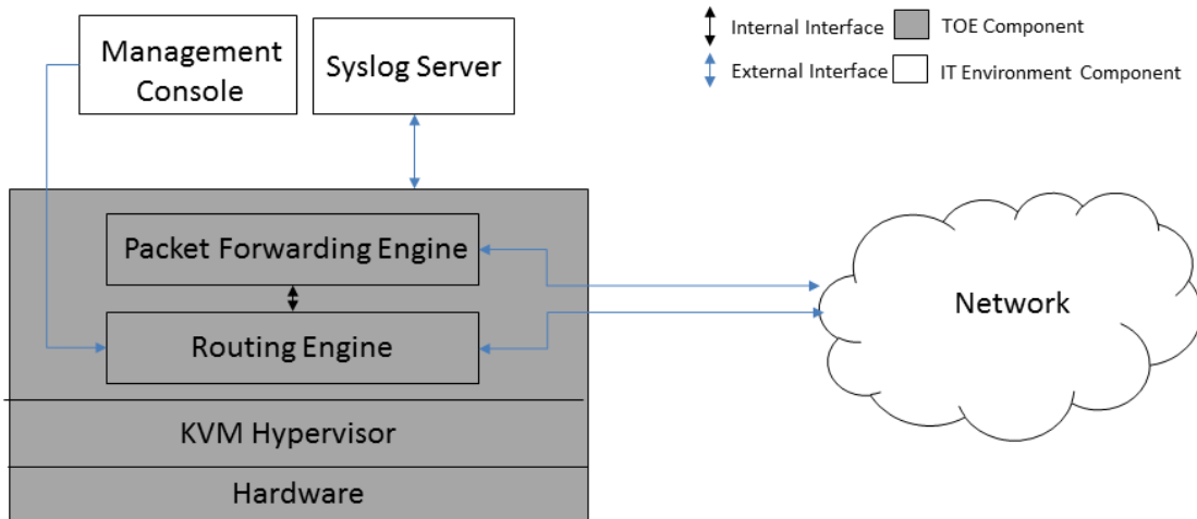
Figure 1 QFX5120, QFX5210, QFX5200 and EX4650 family TOE Boundary
