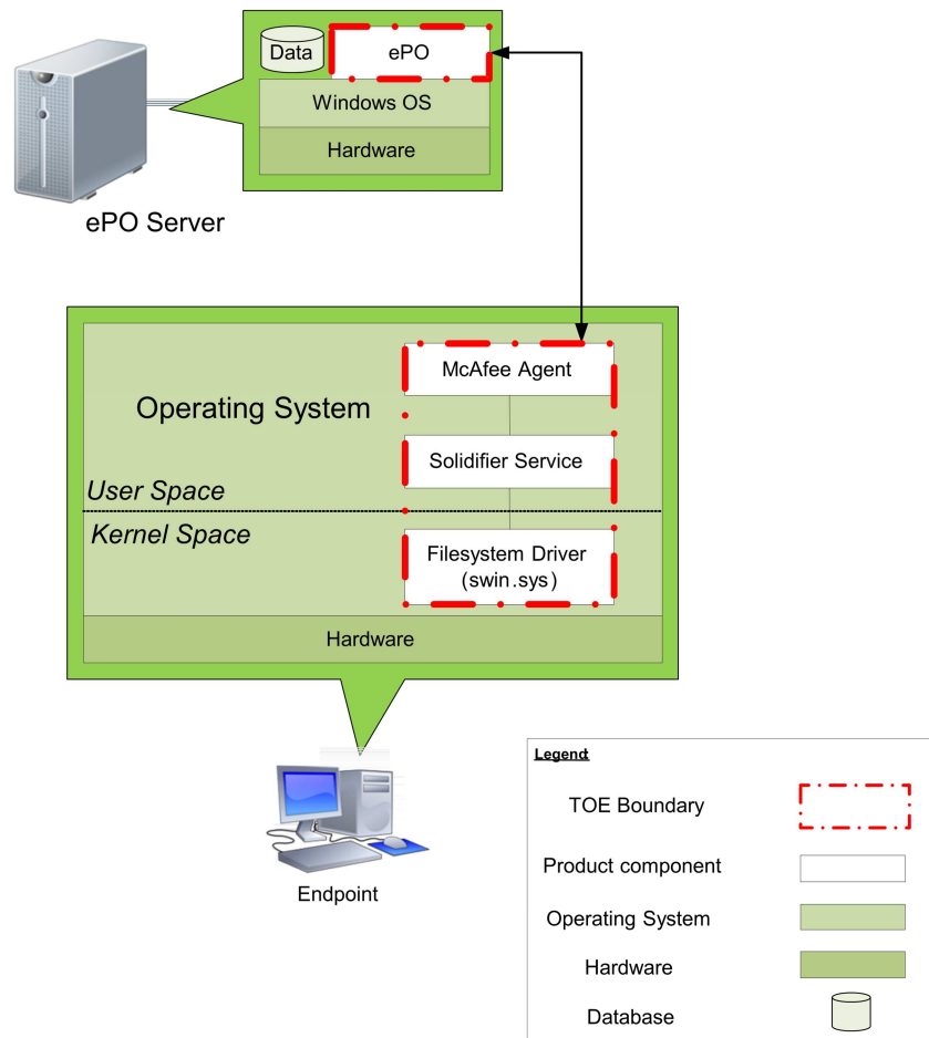
Figure 3 – Physical TOE Boundary
