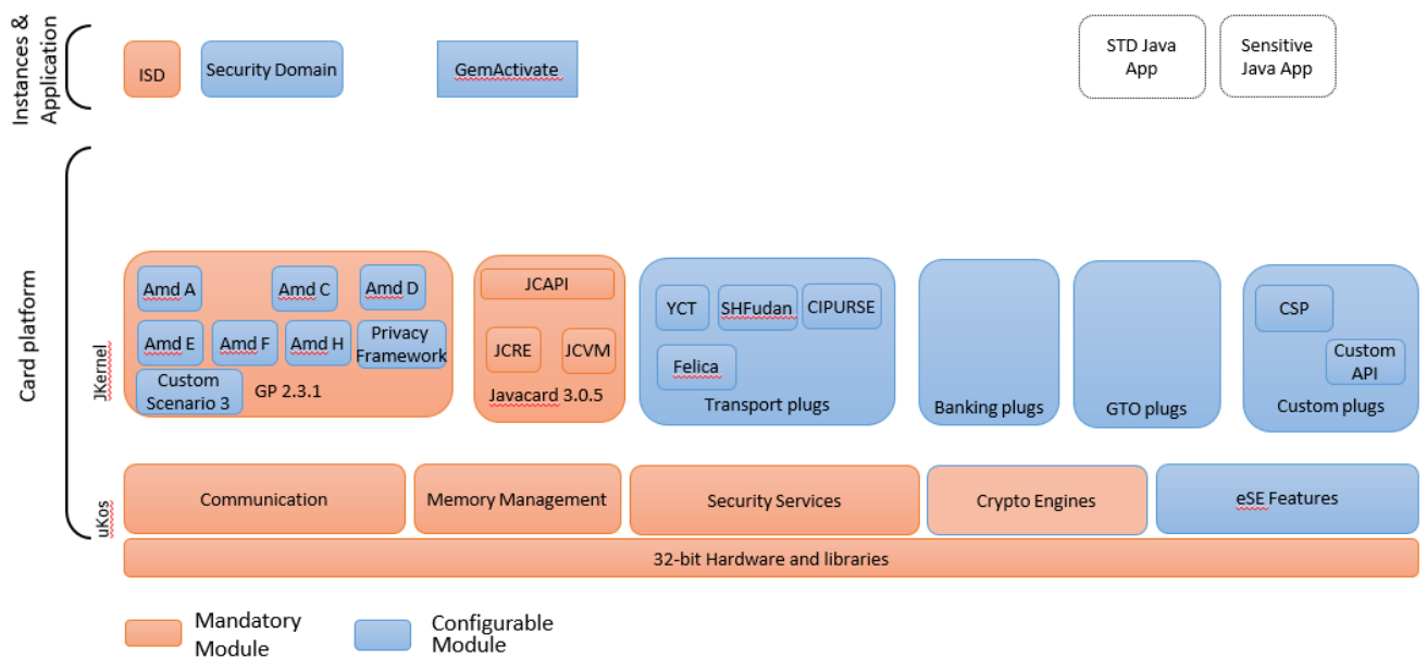
Figure 2: TESS v3.0 on S3NSN4V architecture
