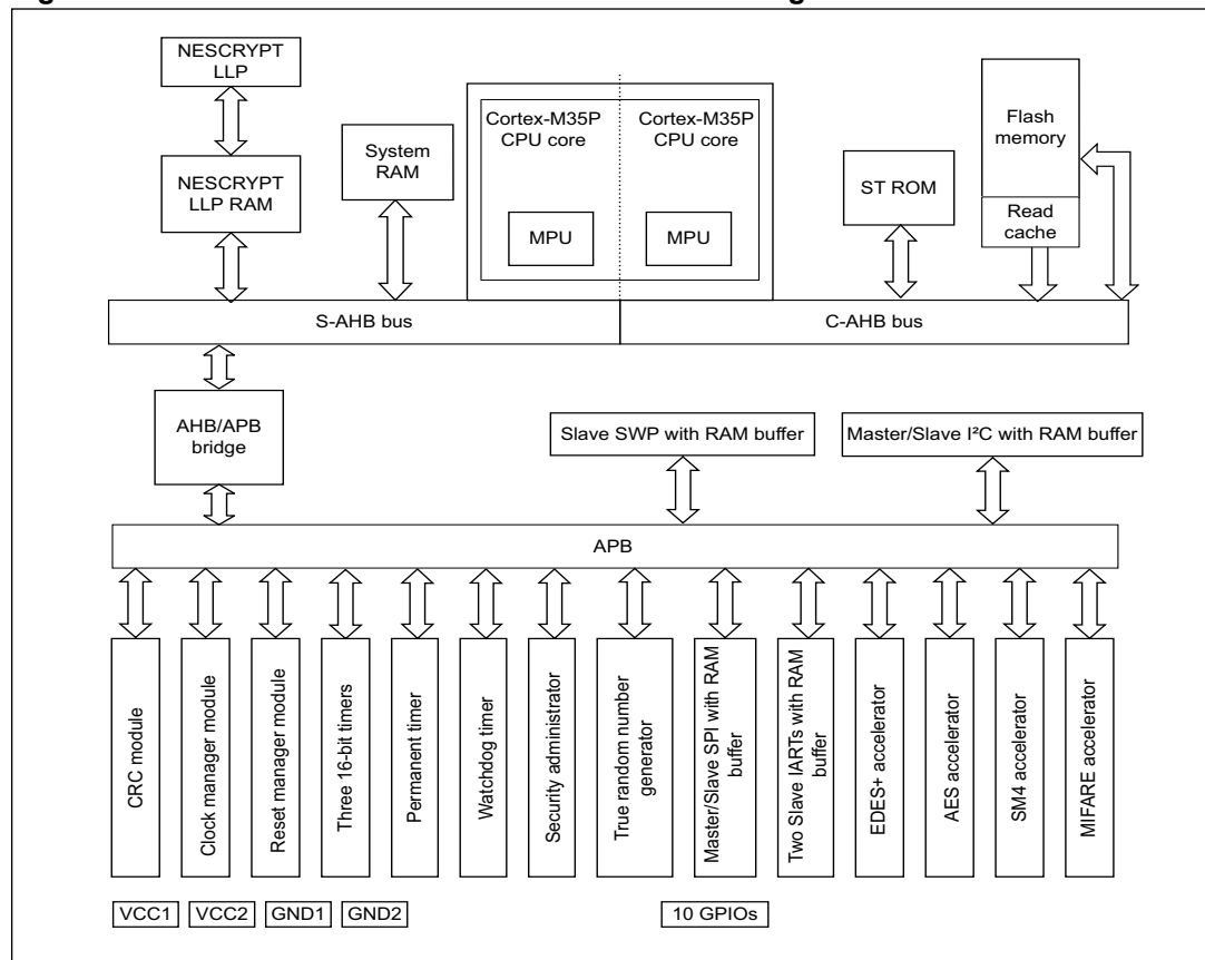
Figure 1. ST33K1M5C and ST33K1M5T C02 block diagram
