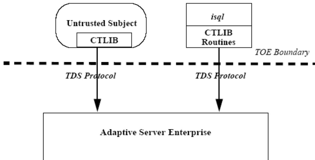
Figure 2 ASE Interfaces
