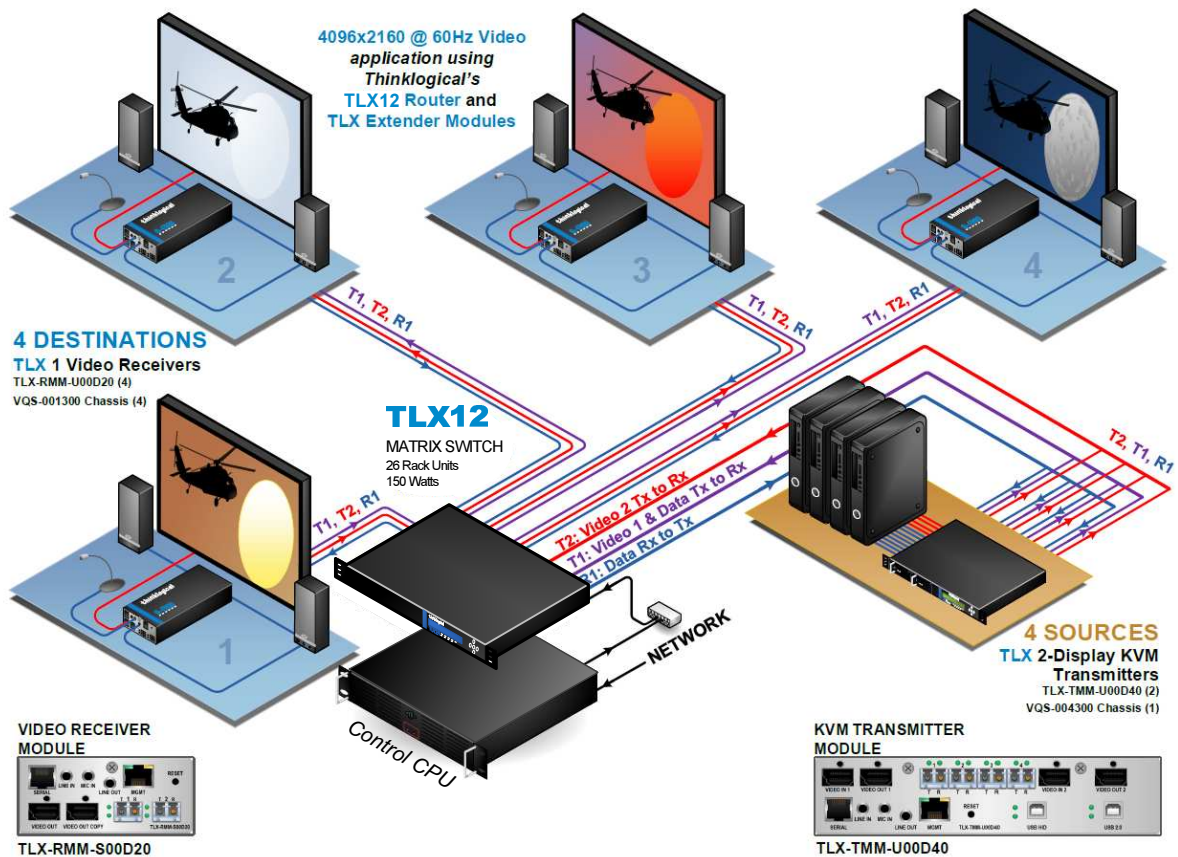
Figure 2b. Typical TOE TLX12 Matrix Switch (w/o Front Control Panel)
