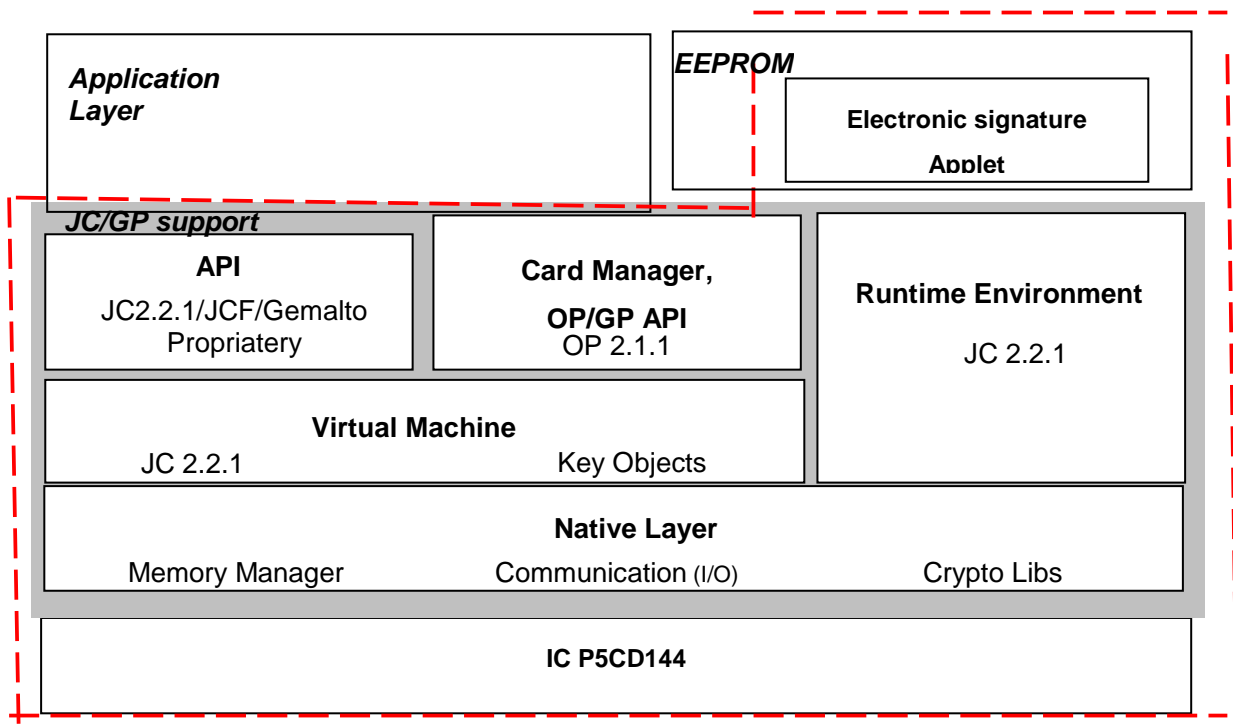
Figure 2 - MultiApp platform architecture
