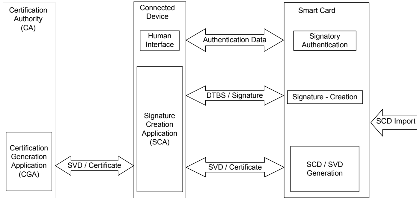
Figure 5 - TOE Usage
