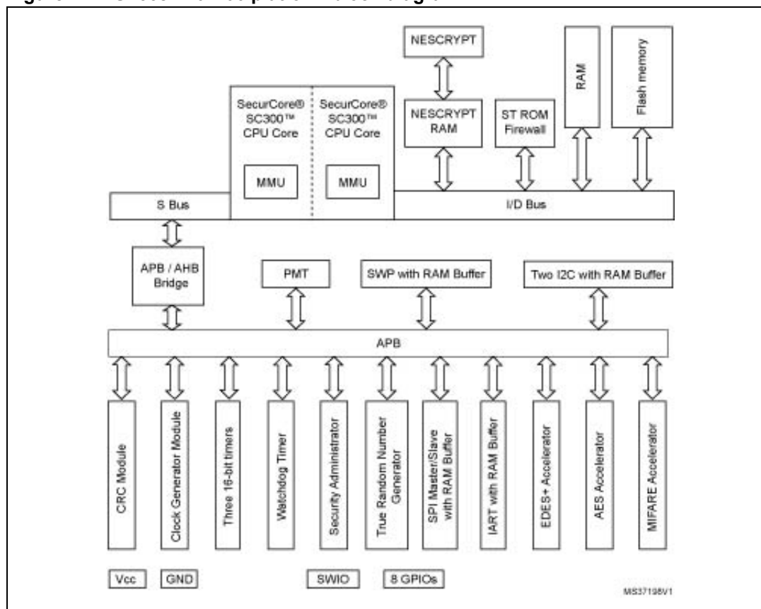
Figure 1. ST33J2M0 A06 platform block diagram
