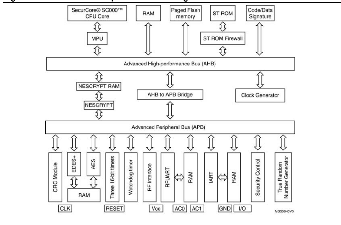
Figure 1. ST31G480 D04 platform block diagram
