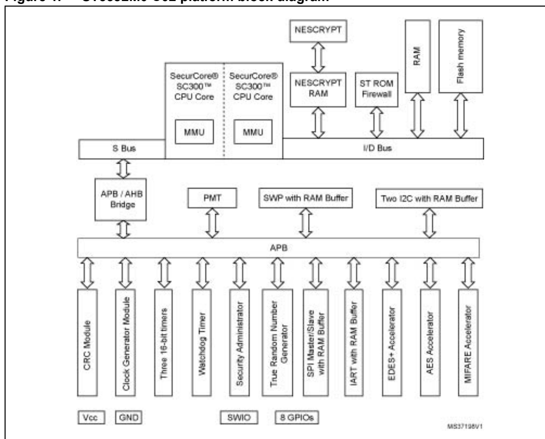
Figure 1. ST33J2M0 C02 platform block diagram
