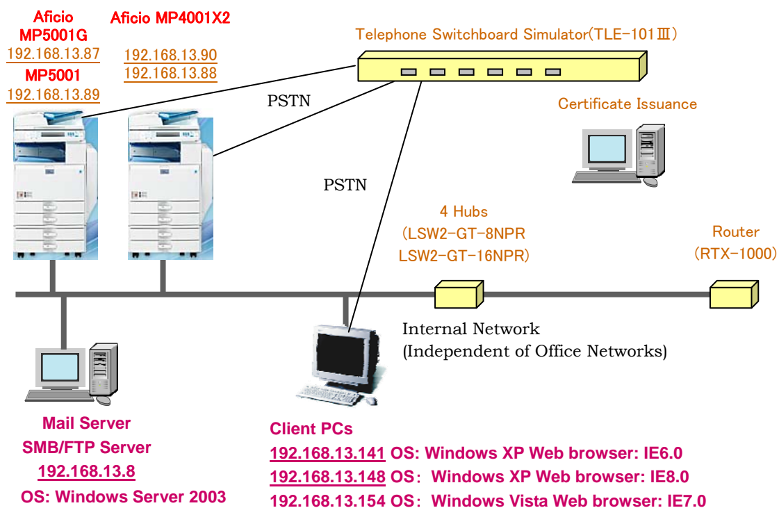
Figure 7-1 Developer Testing Configurations
