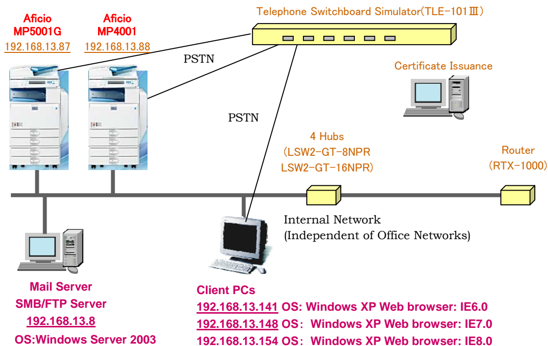
Figure 7-2 Evaluator Independent Testing Configurations
