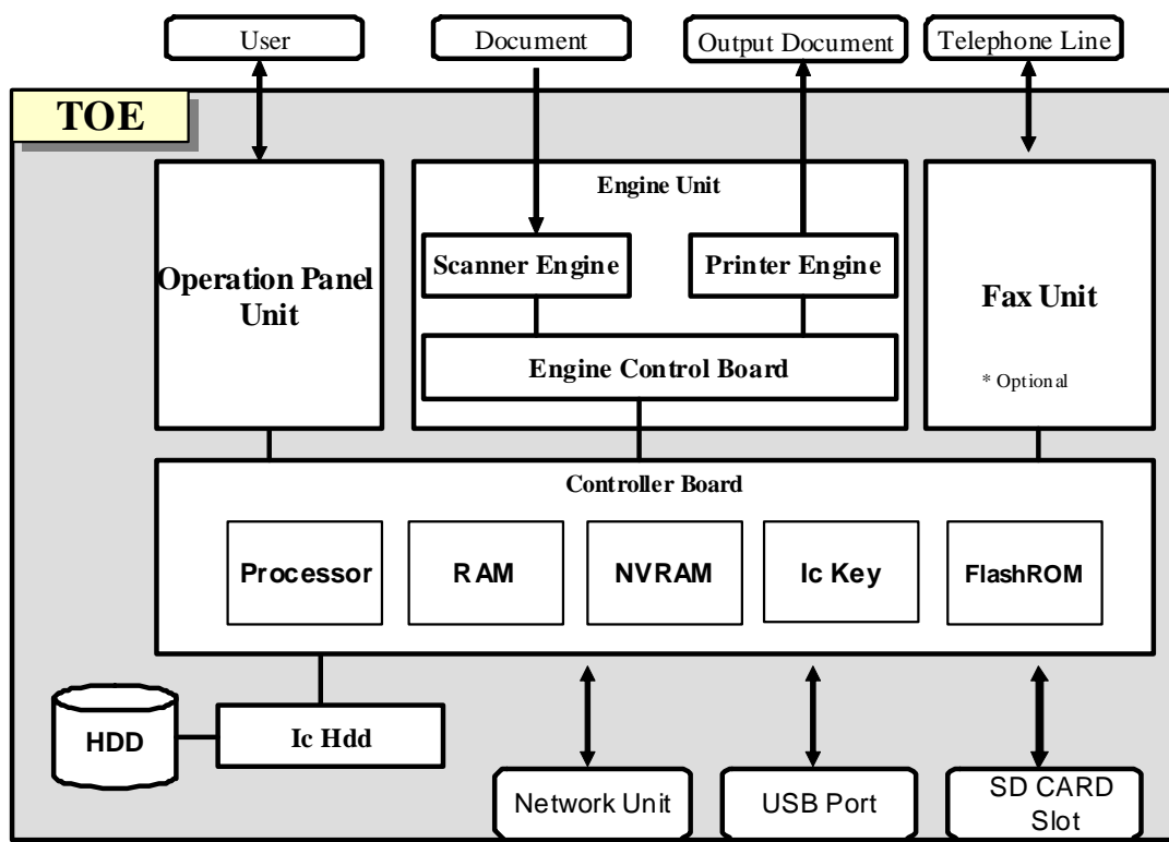
Figure 5.1 TOE boundary
