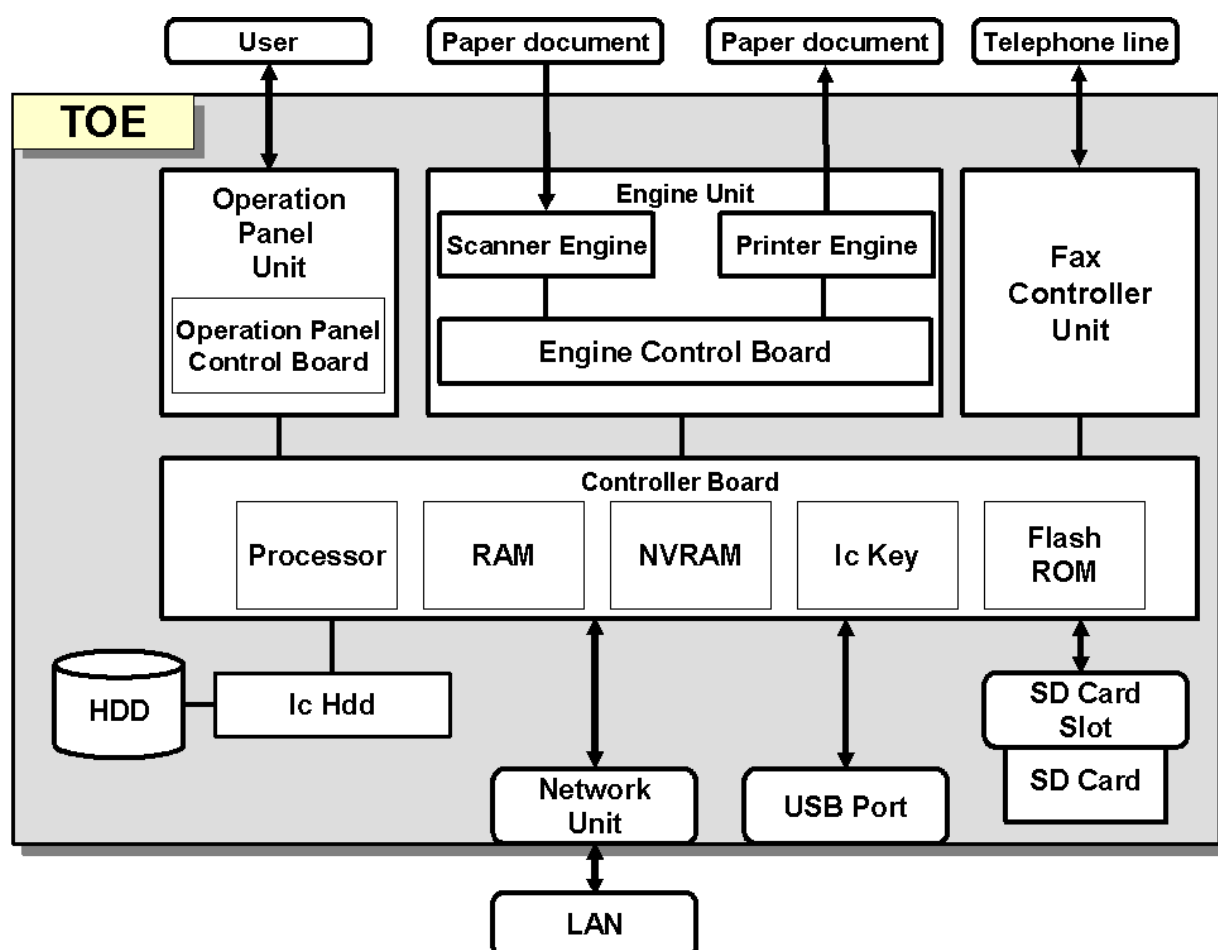
Figure 5-1 TOE boundary
