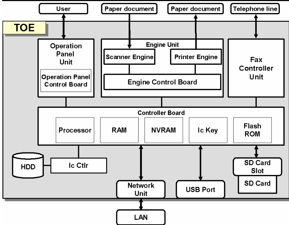
Figure 2 : Hardware Configuration of the TOE
