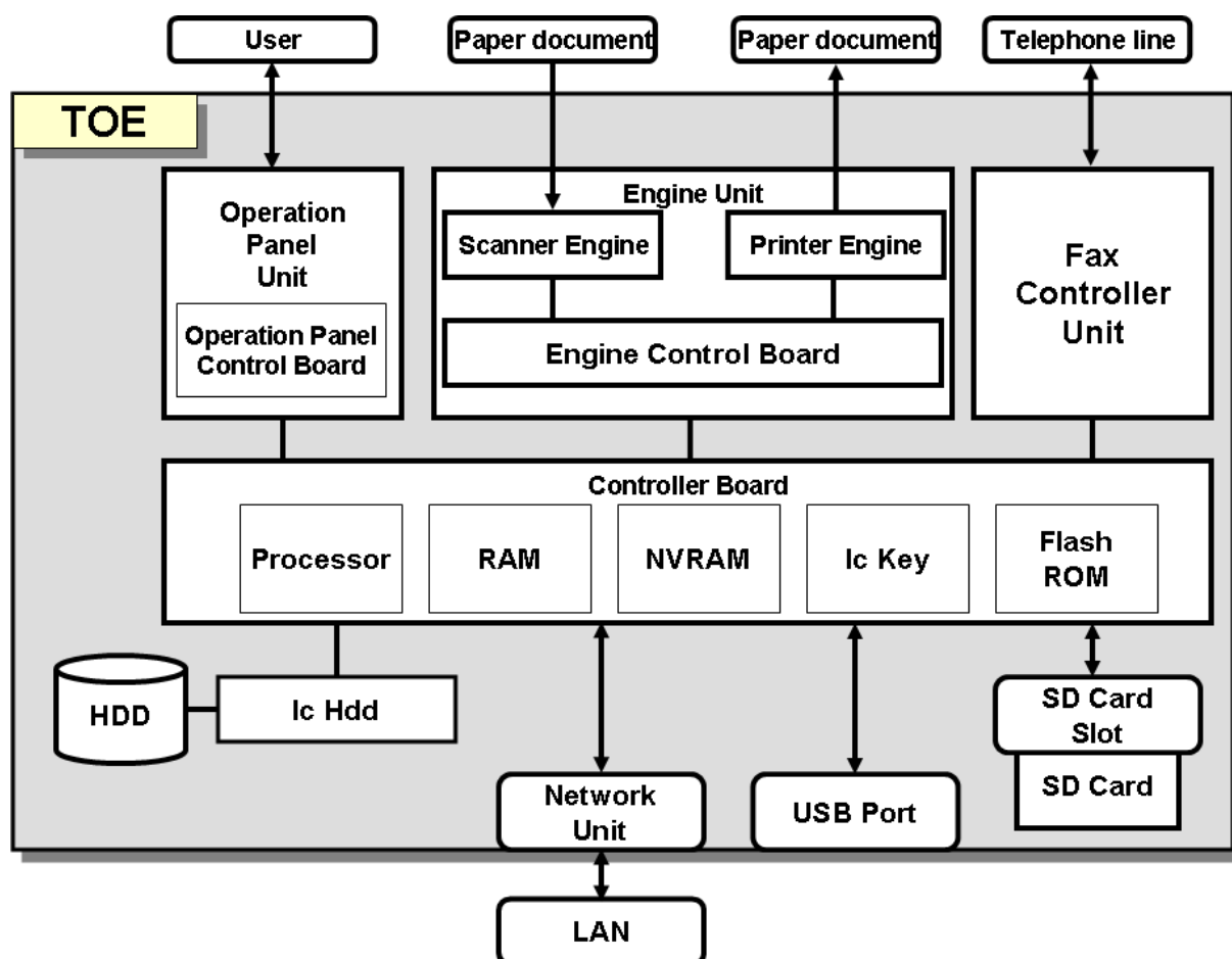
Figure 5-1 TOE Boundary
