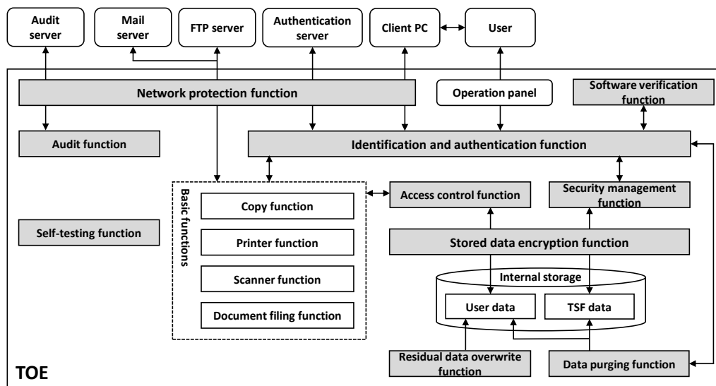
Figure 5-1 TOE boundary
