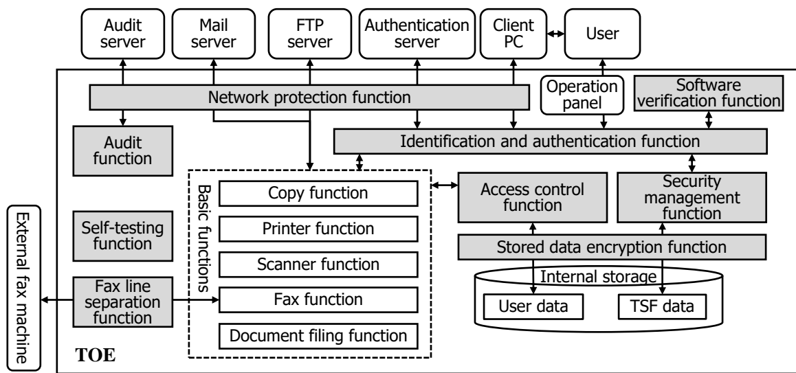
Figure 5-1 TOE boundary
