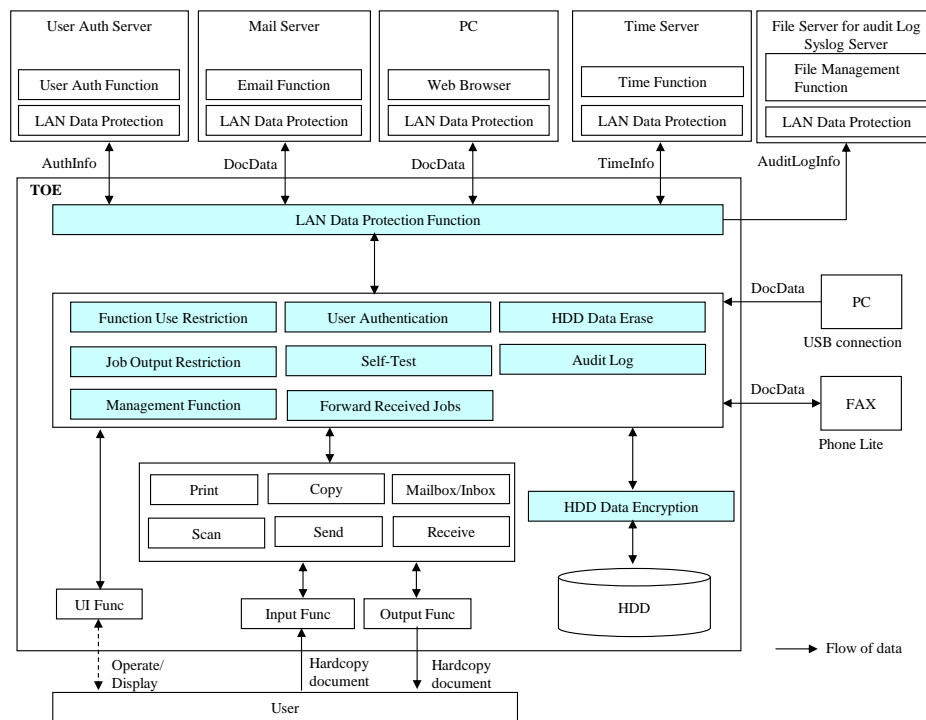
Figure 5-1 TOE Boundary
