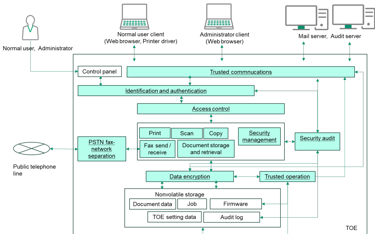
Figure 5-1 Composition of the TOE
