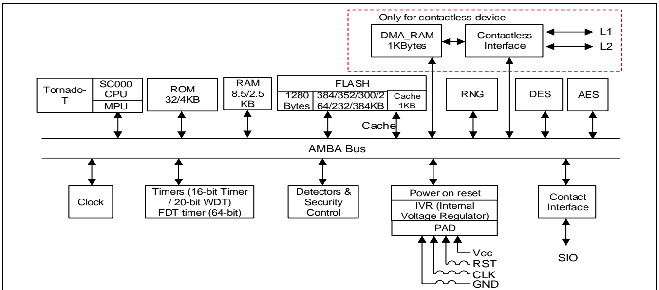
Figure 1 S3D384C/S3D352C/S3D300C/S3D264C/S3D232C/S3K384C Block Diagram
