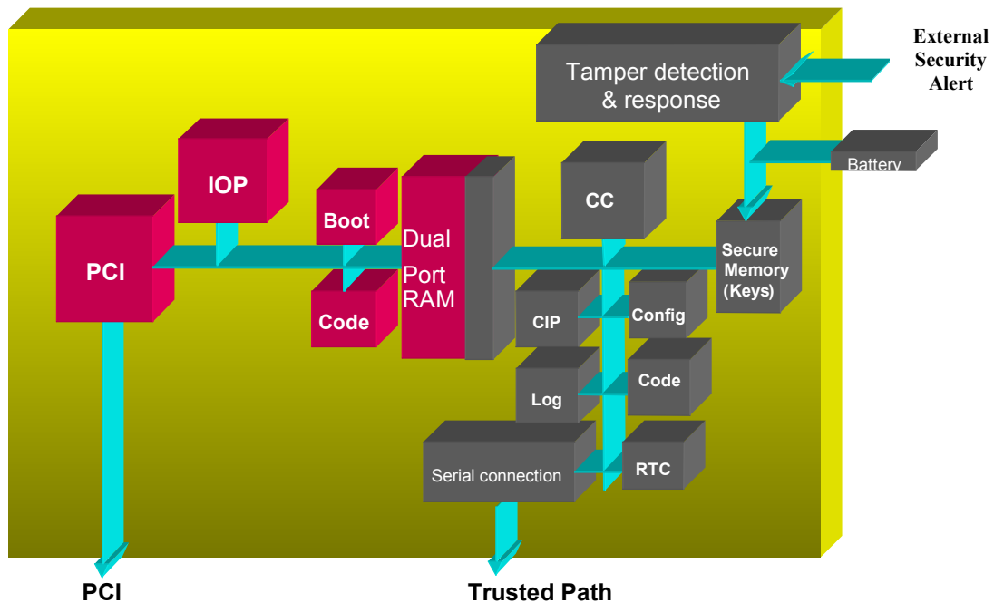
Figure 1: TOE Architecture
