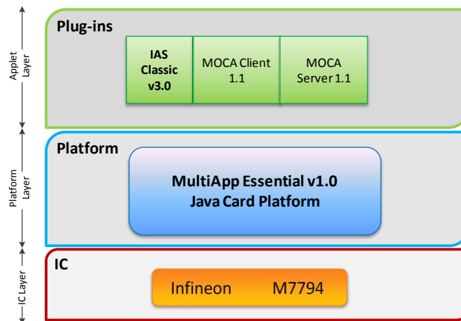
Figure 1: MultiApp Essential V1.0 smartcard architecture
