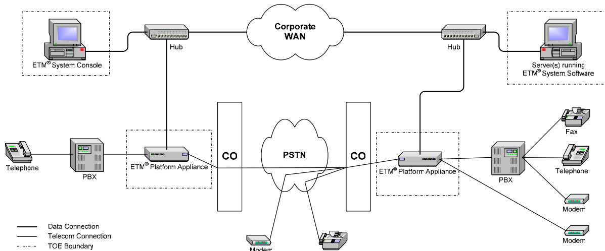
Figure 2: TOE Boundary Diagram
