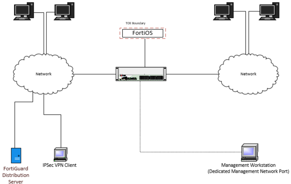
Figure 1 – Single-Unit Configuration
