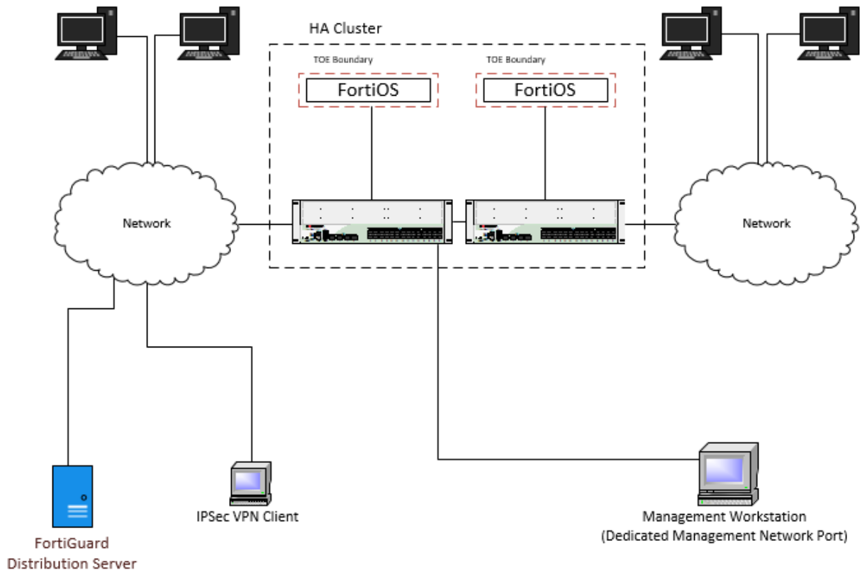
Figure 2 - HA Configuration
