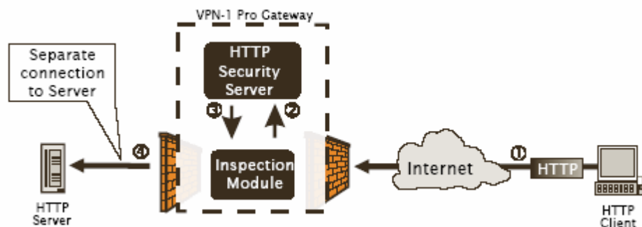
Figure 2-10- Security Servers
