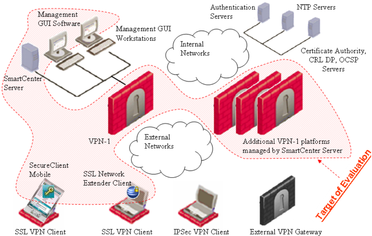
Figure 2 - TOE Architecture
