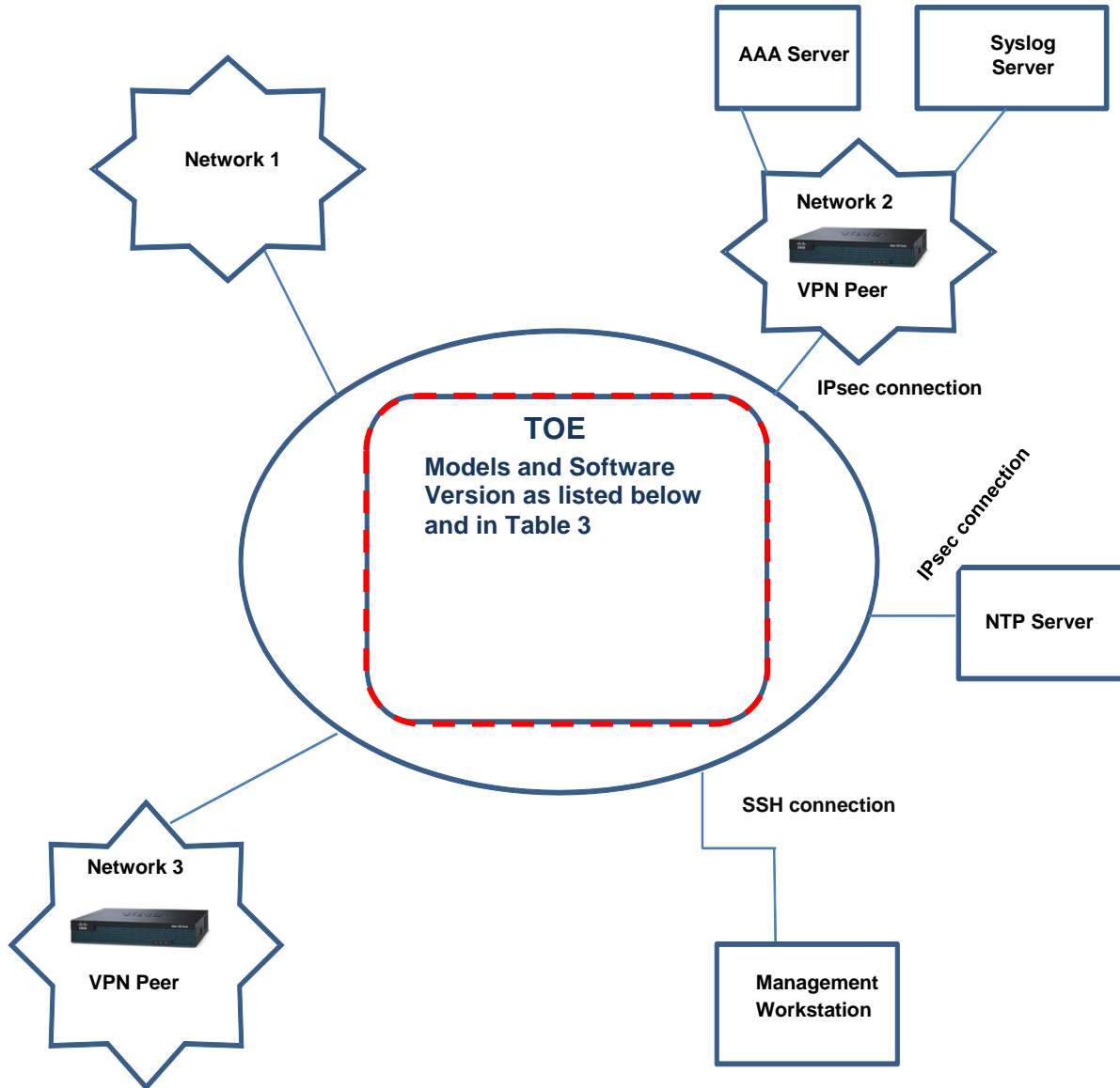
Figure 1 TOE Example Deployment
