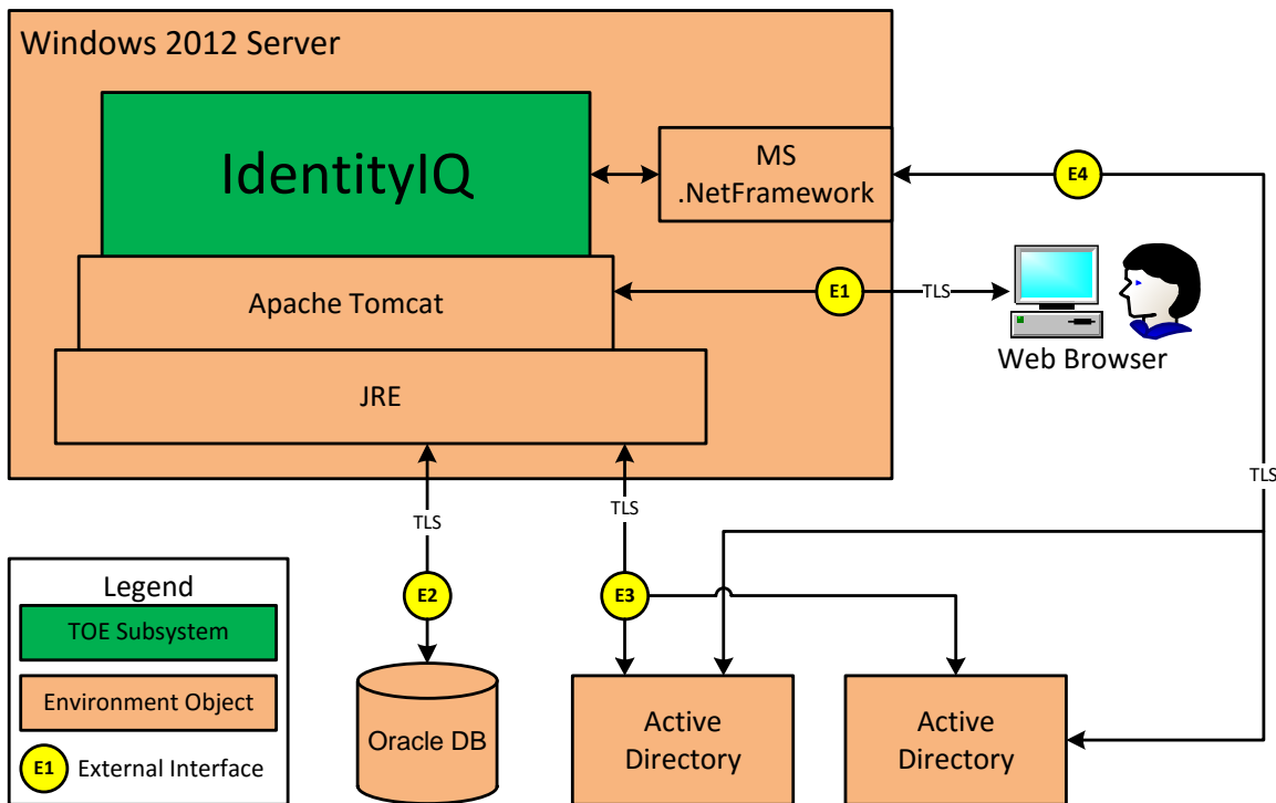
Figure 1-1: TOE Boundary
