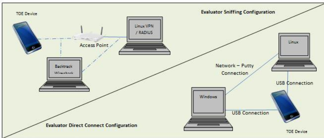
Figure 2 Evaluator Test Setup 2
