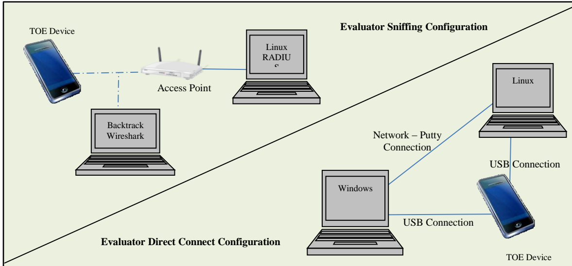
Figure 2 Evaluator Test Setup 2
