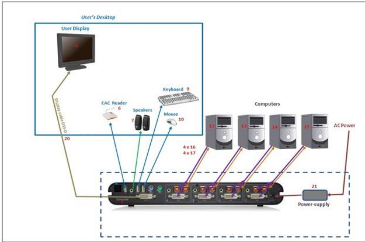
Figure 1: Typical example of a 4-port KVM TOE installation
