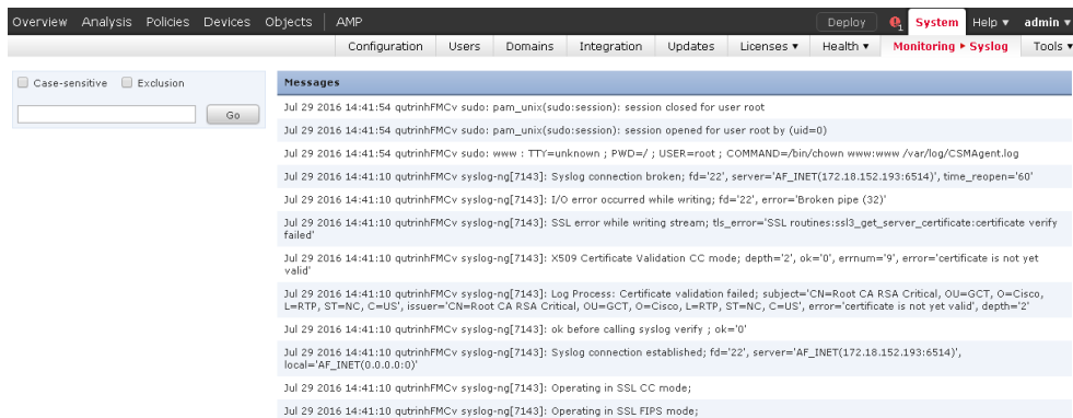
Figure 7: Syslog View
