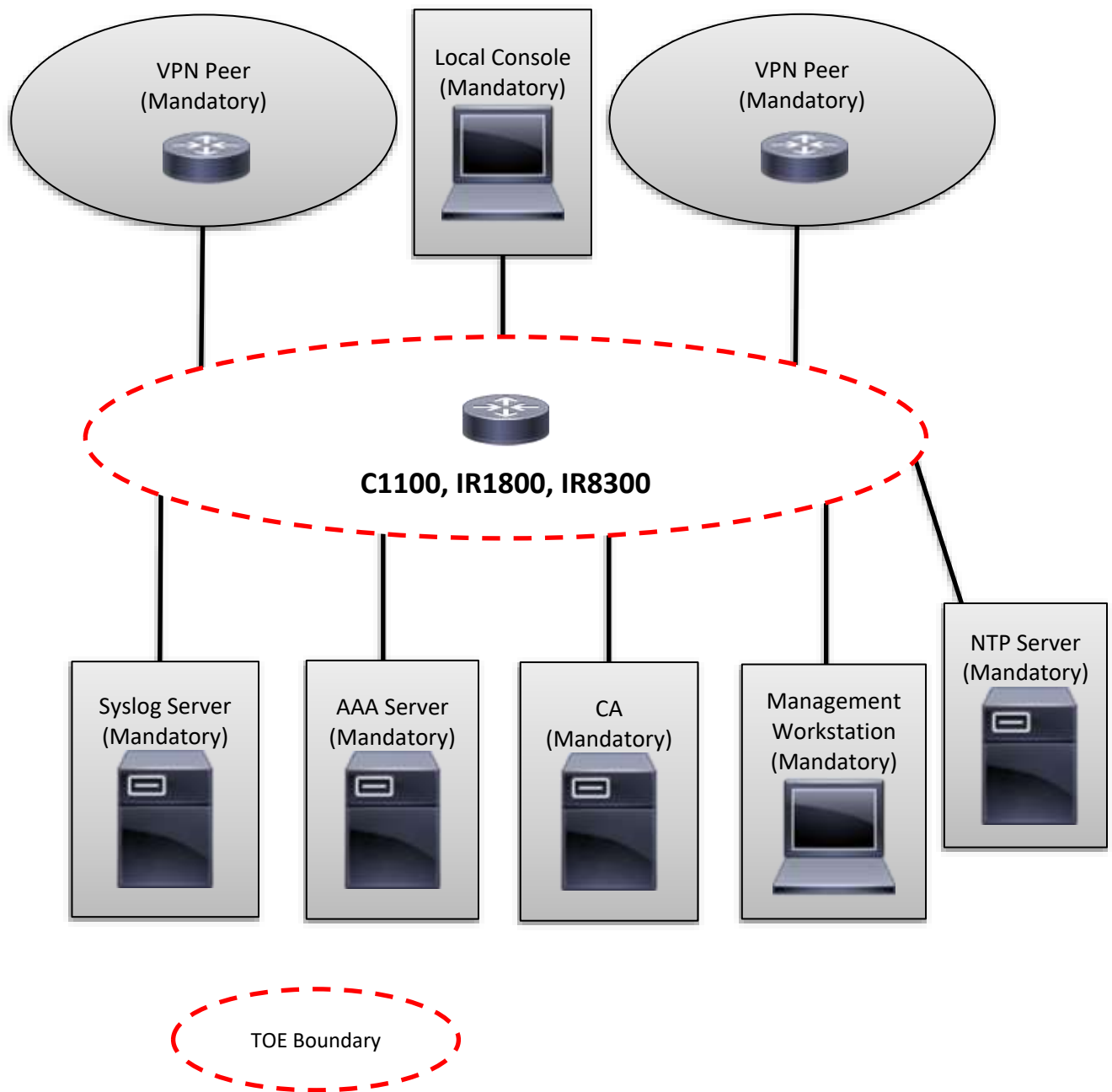
Figure 1 TOE Example Deployment for C1100, IR1800, and IR8300
