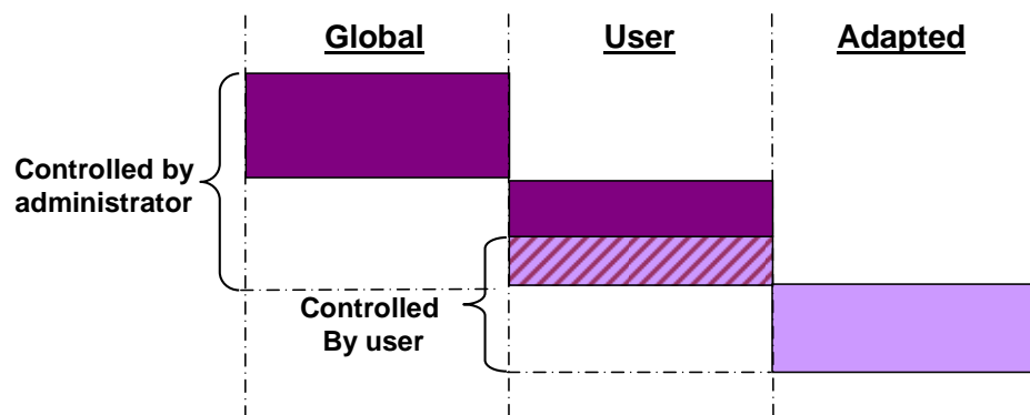
Figure 4: Filtering levels
