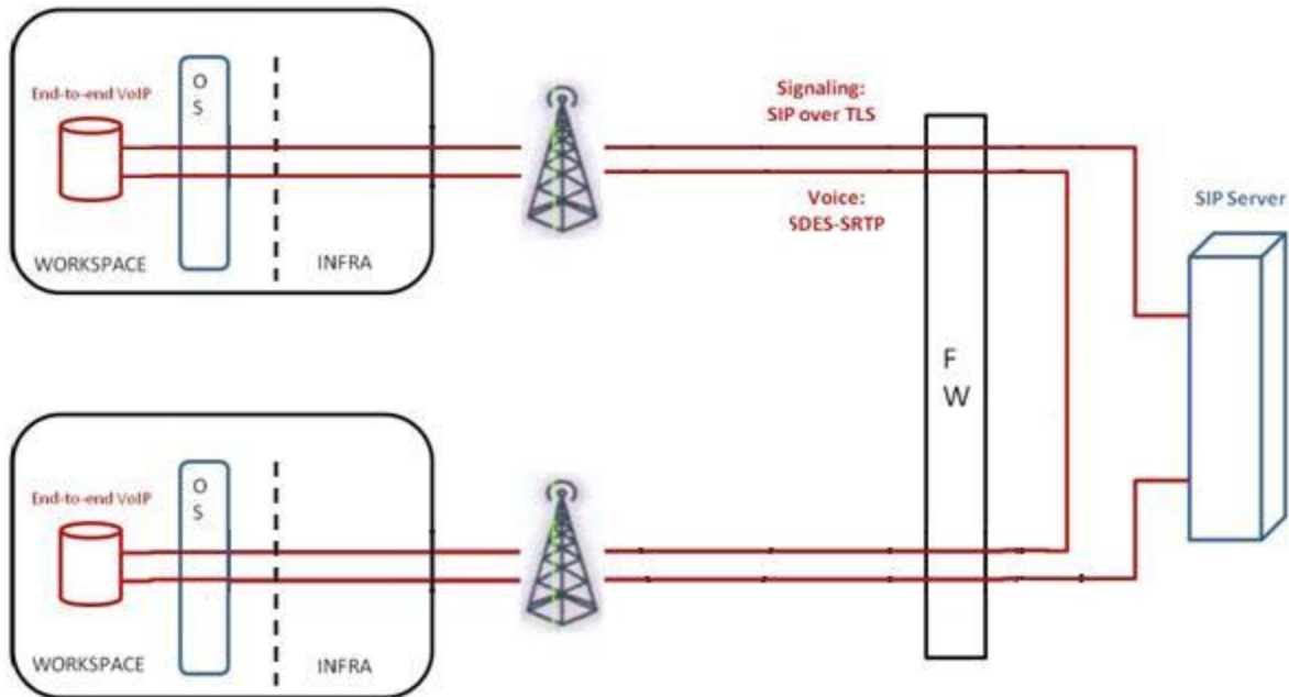
Figure 1: VoIP Communication
